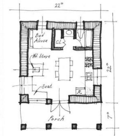
Floor Plan
